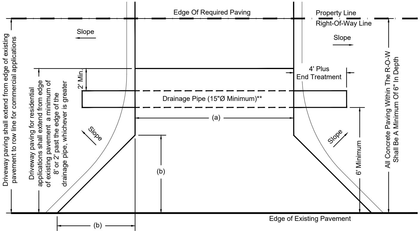
Plan View
